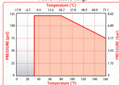
PLC12 Pressure Range
