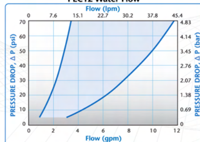
PLC12 Water Flow
